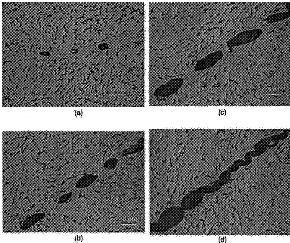
Fig. 8. Void nucleation and growth inside a shear band in Ti–6Al–4V alloy: (a) nucleation of voids within a shear band; (b) growth of voids; (c) elongation and rotation of voids; (d) coalescence.
