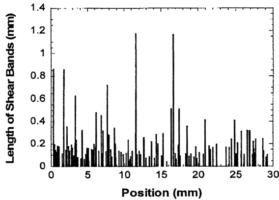
(a) Early Stage, \epsilon_{ef} = 0.55 , L = 0.18 mm, N = 114
