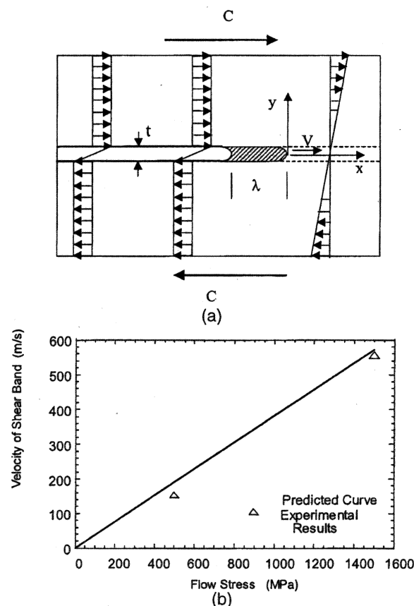
Fig. 12. Calculated propagation velocity for shear band, using Mercier and Molinari's [42] theory: (a) velocity configuration used in calculation; (b) predicted velocities for different conditions.
