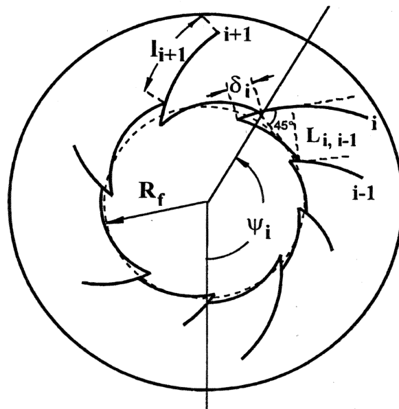
Fig. 4. Characteristics of shear band pattern and basic measurement; \Psi_i is the reference angle and R_f is the final radius of the collapsed cylinder; L_i is the spacing between the i th and the i-1 shear band, l_i is the length of the i th shear band and \delta_i is its edge length.
