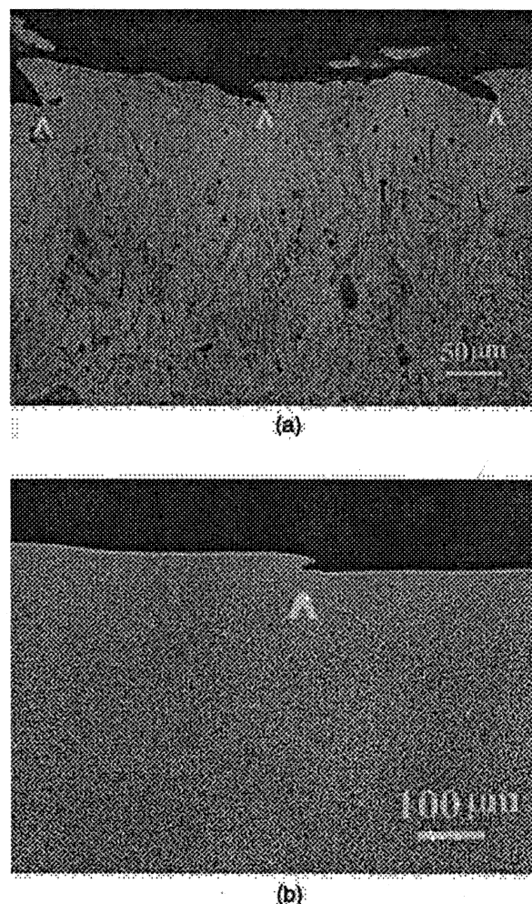
Fig. 5. Comparison of nucleation sites between Ti and Ti-6Al-4V alloy. (a) Titanium and (b) Ti-6Al-4V alloy.
