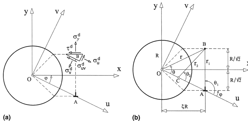
Fig. 14. (a) The shear stress \tau^d along the horizontal slip plane at the point B associated with the stress field \sigma_u^d , \sigma_v^d , and \sigma_{uv}^d of the edge dislocation at the point A . (b) The geometric quantities appearing in the expressions for the stress components at the point B due to edge dislocation at the point A . The lengths \overline{OA} = \overline{OB} = r = \xi R , \overline{OC} = R/\xi , \overline{AB} = r_1 , and \overline{CB} = r_2 . The angle \varphi = \theta/2 .
