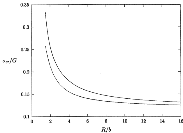
Fig. 16. The normalized critical stress \sigma_{cr}/G required to emit the dislocation from the surface of the void vs. the normalized radius of the void R/b . The upper curve corresponds to emission of the dislocation pair, according to Eq. (27); the lower curve is for the single dislocation, according to Eq. (13). The calculations are for \rho = 1 and \nu = 1/3 .
