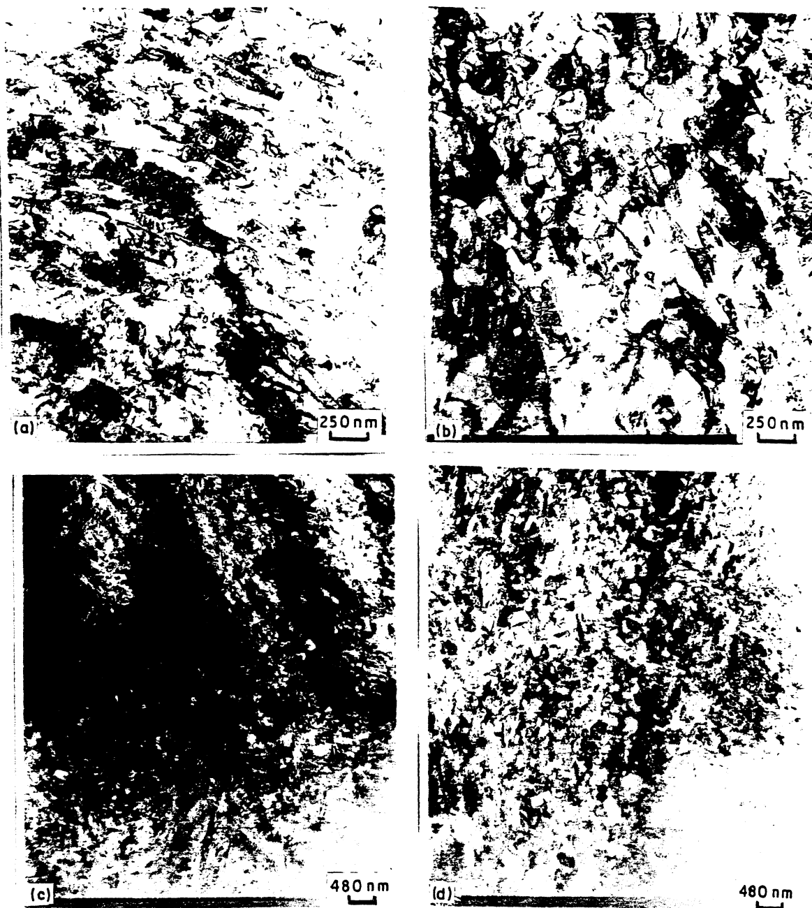
Figure 13 (a) and (b) Regions affected by interparticle heating; (c) region exhibiting laths; (d) boundary between heat-affected and shock hardening region.
