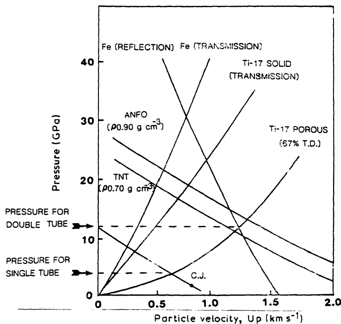
Figure 3 Pressure versus particle velocity curves leading to determination of pressures for single-tube and flyer-tube techniques.
