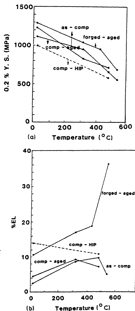
Figure 14 Variation of (a) yield stress and (b) total elongation with temperature for Ti-662 in shock-consolidated, shock-consolidated + aged (570°C per 4 hr), shock-consolidated + HIPped conditions; forged + aged (570°C for 4 h) material given as comparison.
