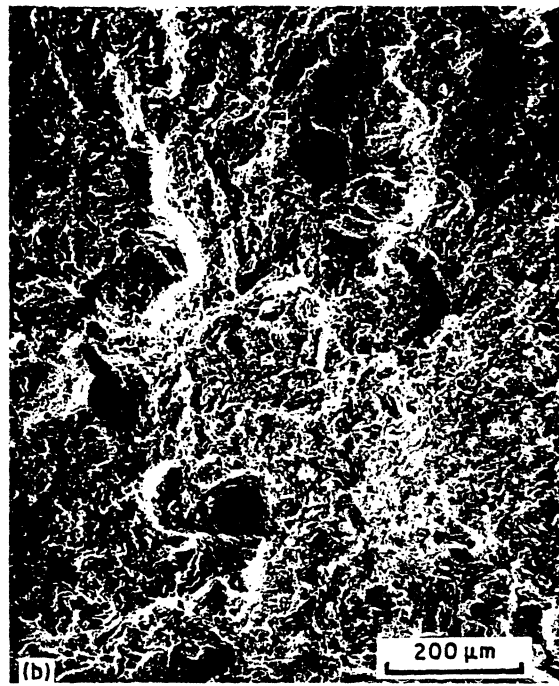
Figure 15 (a) Scanning electron fractograph of poorly shock-consolidated material; notice easy separation at particle interfaces. (b) Scanning electron fractograph of well consolidated material; the dimple morphology is characteristic of the ductile fracture mode (interparticle).
