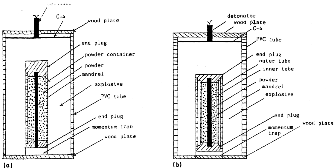
Figure 2 Systems used for shock consolidation of titanium alloys. (a) single tube, (b) double (or flyer) tube.
