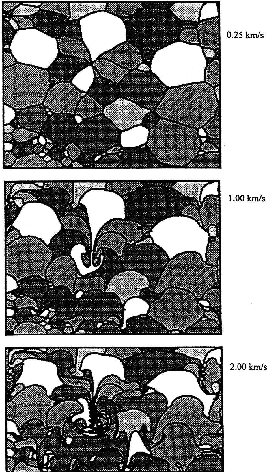
Fig. 17. The final configurations for the cylindrical particles of Inconel 718 with an initial porosity of 19% and particle velocities of 0.25, 1.00, and 2.00 km/s.
