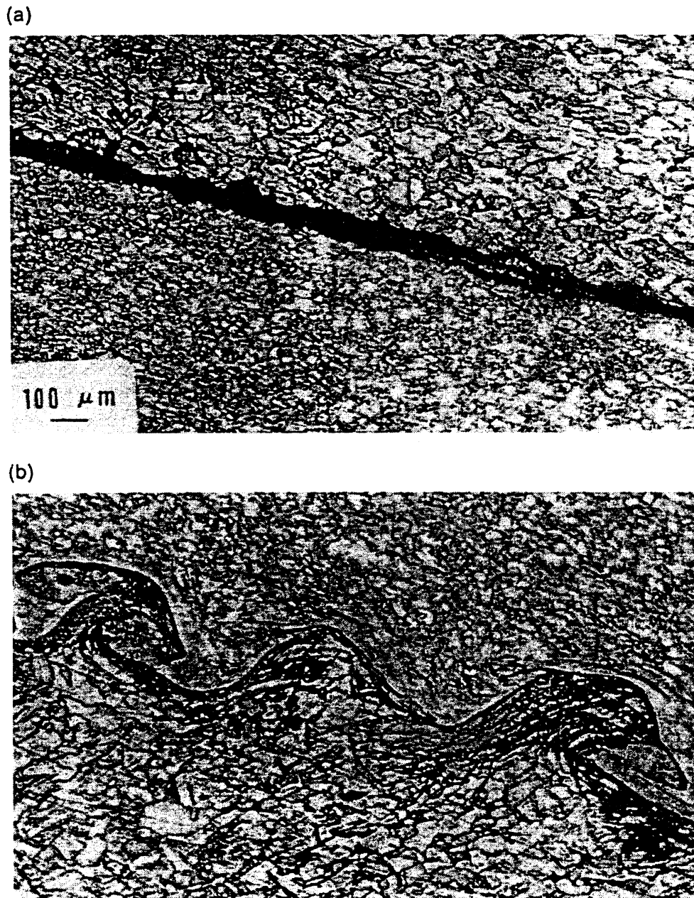
Fig. 10. Appearance of interface in model experiment of Fig. 9: (a) central region which underwent normal impact; (b) lateral region.
