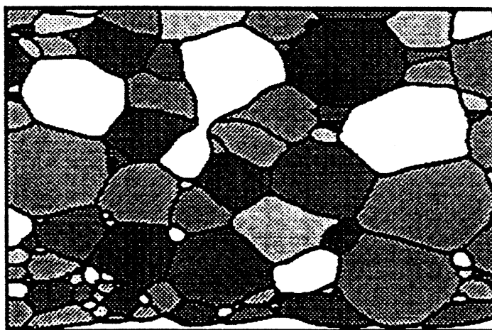
Fig. 18. The final configurations of SiC with an initial porosity of 19% and particle velocities of 0.5, 1.00, and 2.00 km/s.
