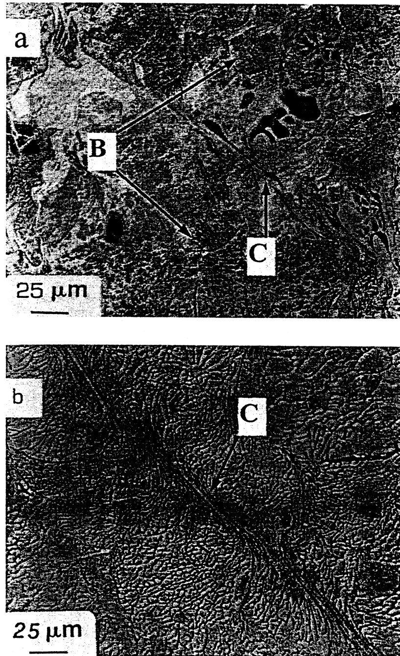
Fig. 6. Optical micrographs showing localized shear deformation (C) and interparticle melting (B) along the shear zone in \text{Ti}_3\text{Al} alloy compact.
