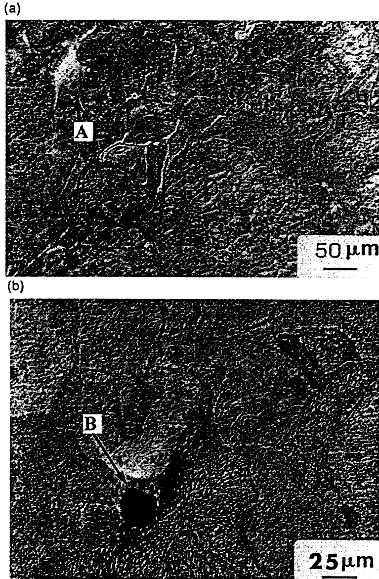
Fig. 3. Optical micrographs of shock-consolidated \text{Ti}_3\text{Al} showing evidence of melted and rapidly solidified material (A) and shrinkage void at the center of melting pool (B).
